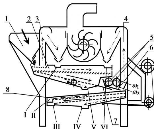
Figure 1. Process diagram of a flax seed separator: (1) feeding hopper, (2,8) screen shoe, (3,4) pneumatic ducts, (5) threshing device, (6,7) chutes, (I,VI) chute of light impurities, (II) chute of heavy impurities, (III) chute of flax seeds, (IV) and (V) chute of fine impurities, movement direction of: \longrightarrow – mass, \cdots\cdots\longrightarrow – light impurities, -\ -\longrightarrow – seed-bags, \longrightarrow – bulk seeds, - \cdot \longrightarrow – fine impurities.
